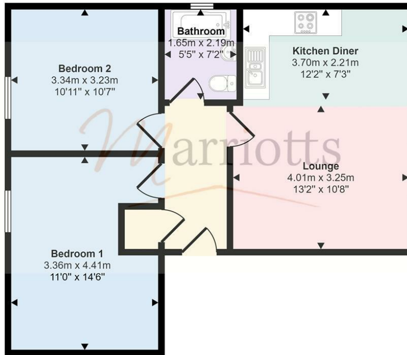
Floorplan
